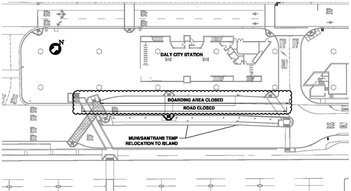
FIGURE 2: BUS STOP RELOCATION DURING WORK AT WESTERN LANES
